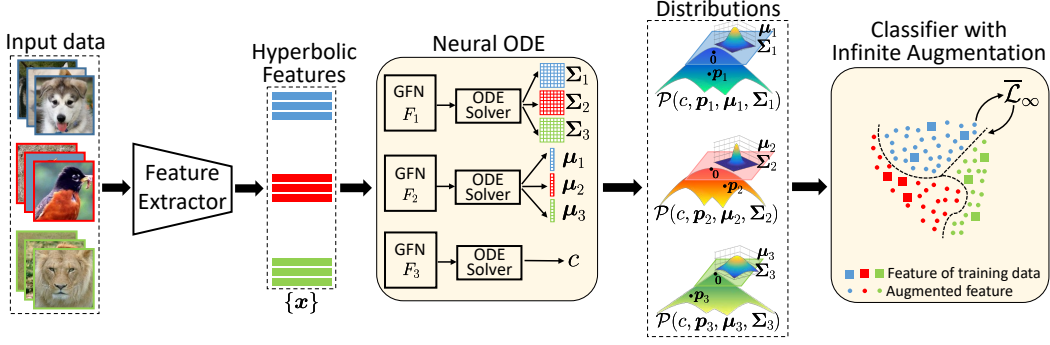
Figure 1: A conceptual diagram of HFA. GFN denotes the proposed gradient flow network.
