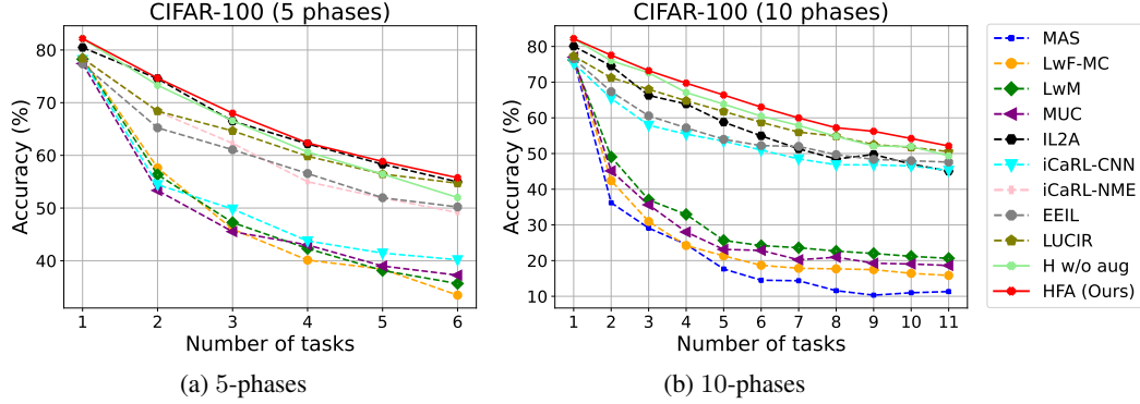
Figure 4: Top-1 accuracy on CIFAR-100 in continual learning.
