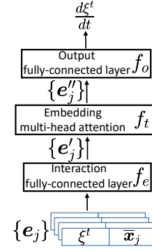
Figure 2: Architecture of the gradient flow network.
